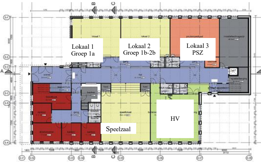
begane grond 1:200
